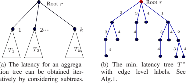
Fig. 2. Latency of aggregation along a tree.
