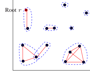
Fig. 1. Example of a function dependency graph \mathcal{G} and the function decomposes in terms of the maximal cliques of the graph, as represented by dotted lines.
